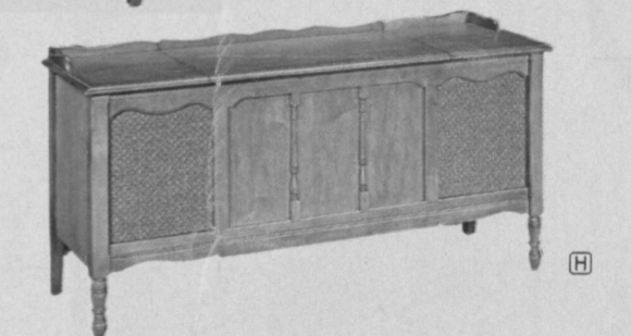
H The HUMBOLDT • X924M Early American styled cabinet in genuine Maple veneers and solids. Center lift lid; record storage space. Six high-fidelity speakers (two large 10" woofers and four 3 1/2" cone-type tweeters) with Alnico-5 magnets. Zenith Stereo Precision 4-speed automatic record changer with Micro-Touch® 2G tone arm. Cabinet size: 26" high, 52" wide, 17" deep.
