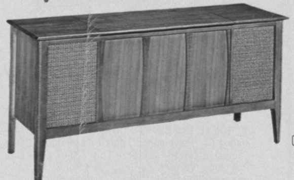
I The LISZT • X920W Danish Modern styled cabinet in genuine oil finished Walnut veneers and select hardwood solids. Lift lid; record storage space. Six high-fidelity speakers (two large 10" woofers and four 3 1/2" cone-type tweeters) with Alnico 5 magnets. Zenith Stereo Precision 4-speed automatic record changer with Micro-Touch® 2G tone arm. Cabinet size: 25" high, 52" wide, 17" deep.
