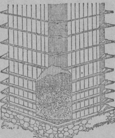
CONSTRUCTION OF A SQUARE SILO.
